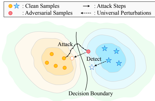
Figure 1: Illustration of our UAPAD framework. The solid and hollow markers represent samples before and after the universal perturbation. The adversarial samples are embedded closer to the decision boundary to maintain similarity with the original samples, resulting in differential resistance to universal adversarial perturbations (UAPs) with clean samples. We construct our detection framework based on this observation.
