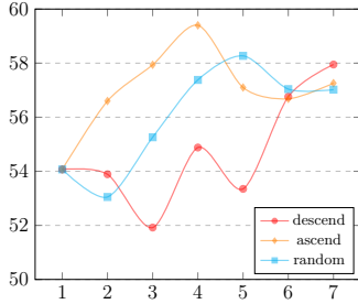
Figure 1: Changes of F1-score as more source domains are introduced in three different orders: descending order (red), ascending order (orange) and random order (blue) of EECR scores.
