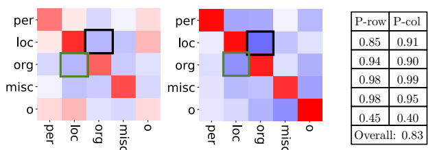
(a) Consistency: CoNLL (b) Error: CoNLL (c) Pearson coefficient
